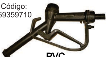
PVC Conector: 3/4" - Pico: 20 mm
